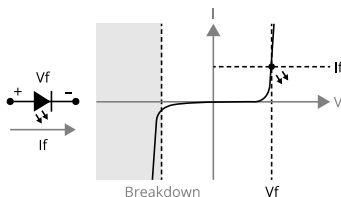
LED Symbol & Voltage vs Current Graph
